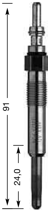
Y-732 J M 10 x 1.0 10 Hex 12 V DP 4
