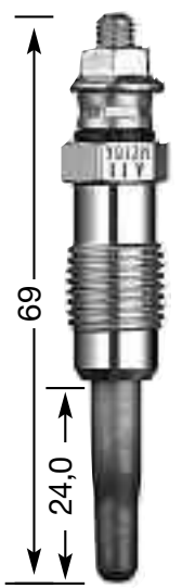
Y-913 M M 12 x 1.25 12 Hex 11 V
