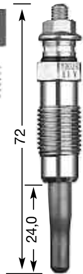
Y-902 R M 12 x 1.25 12 Hex 11 V
