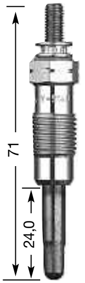
Y-914 U M 12 x 1.25 12 Hex 11 V
