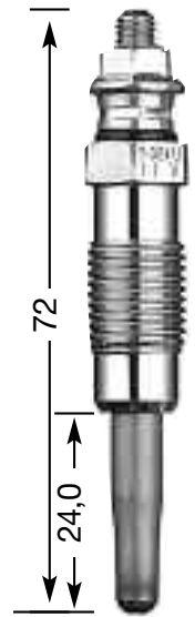
Y-924 U M 12 x 1.25 12 Hex 11 V
