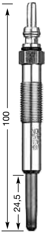
Y-516 J M 10 x 1.0 10 Hex 11 V DP 12
