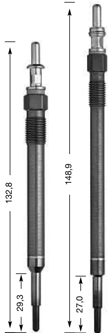
CZ 106 M 10 x 1.0 10 Hex 7 V DP 53
