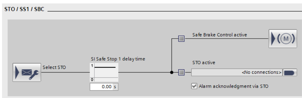
Рисунок 10-8 Safety Integrated Basic Functions STO, SS1, SBC
