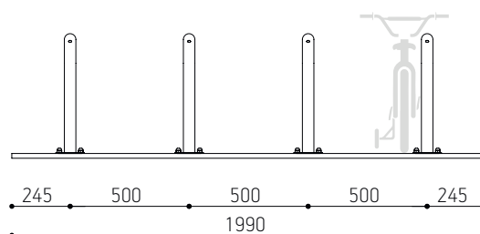
Kaar Mini bicycle parking, with 4 arches KM300-4
