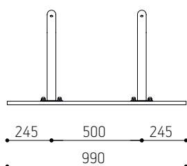
Kaar Mini bicycle parking, with 2 arches KM300-2
