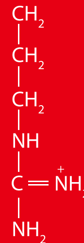
Arginine
